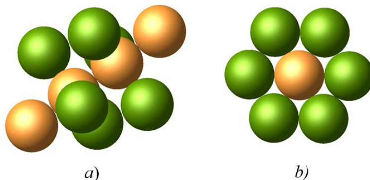
Fig. 4. A simple model of electron shells for the first 10 electrons in two projections: a) in a plane passing through the axis of rotation of the atom at an angle of 45^{\circ} ; b) in a plane perpendicular to the axis of rotation and passing through the center of the nucleus. ● – s -electrons, ● – p -electrons
