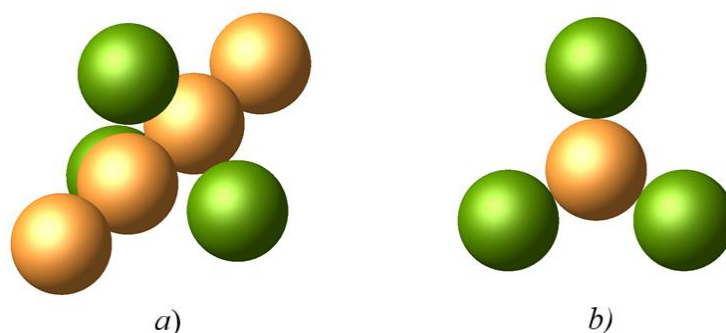
Fig. 3. Model of electron shells for Z = 7 in two projections: a) in a plane passing through the axis of rotation of the atom at an angle of 45^{\circ} ; b) in a plane perpendicular to the axis of rotation and passing through the center of the core. ● – s -electrons, ● – p -electrons
